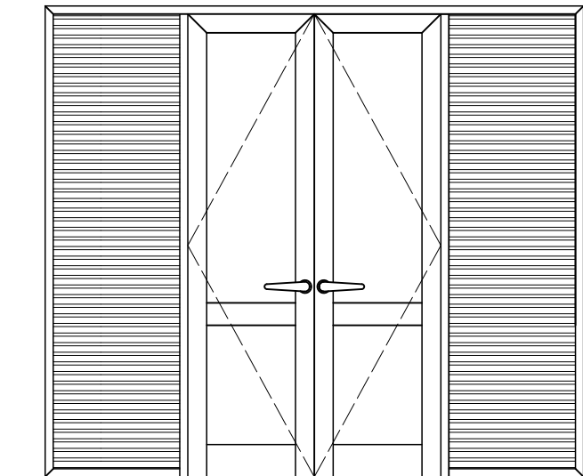
Side Louvre
