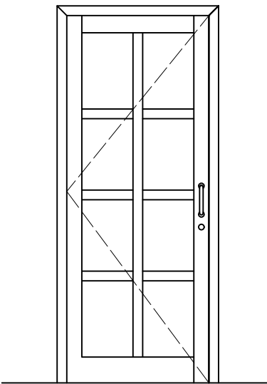
Divided sash
