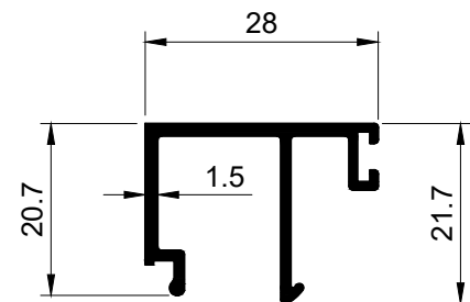
SECTION NO. - GL-116 EST. WEIGHT - 0.299 KG./M. GLASS GAP - 12.5 MM
