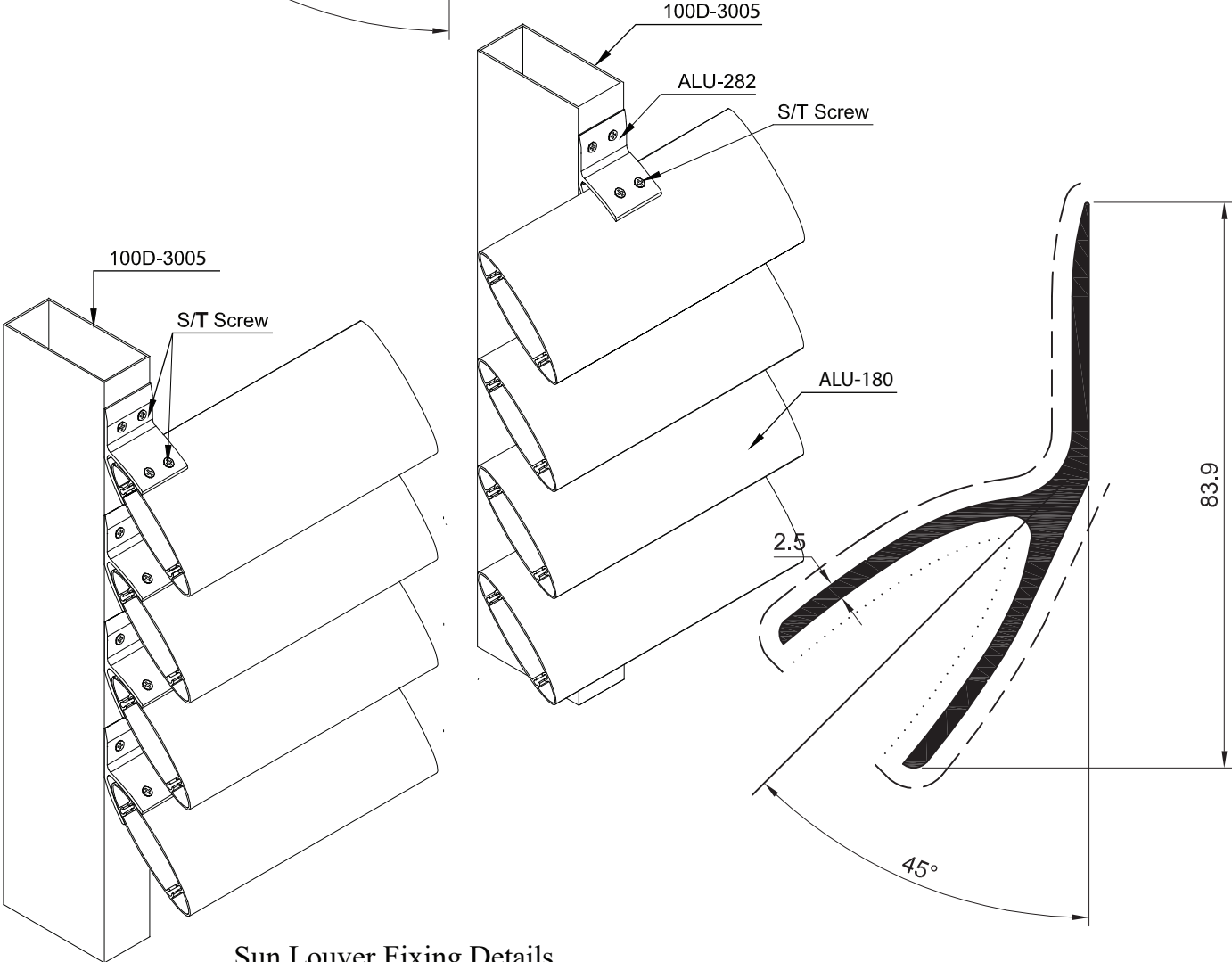
Sun Louver Fixing Details
